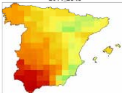
ECHAM4_A2_INM 2011_2040
