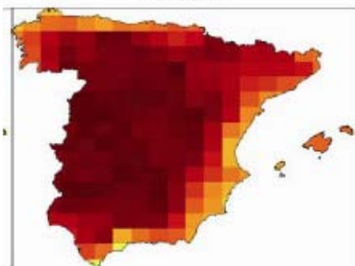
ECHAM4_A2_INM 2071_2100
